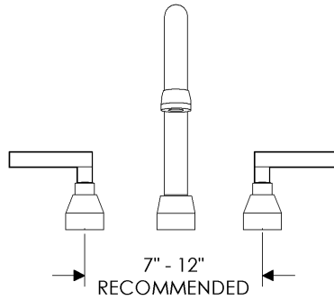
DMF Deck Mount Faucet & Rough with P605 spout.
